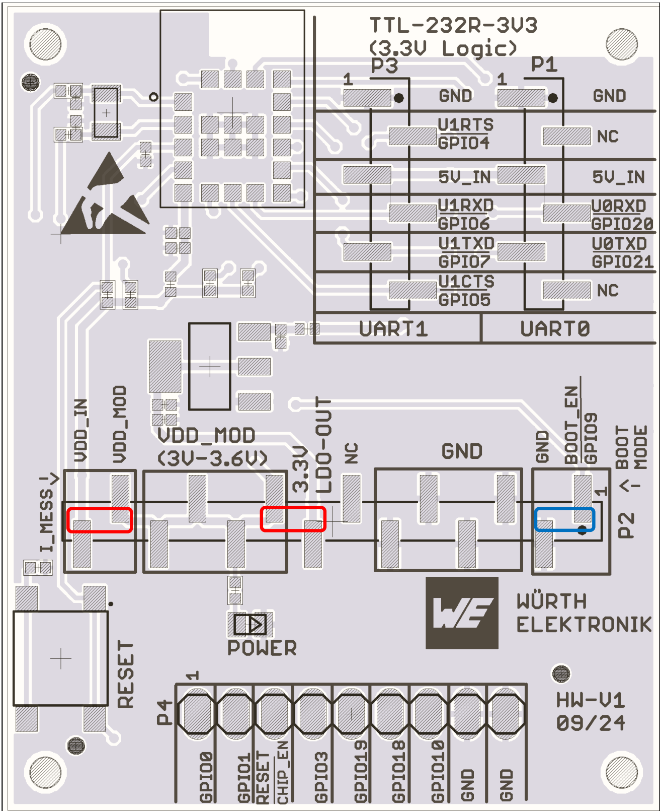
Figure 6: Jumpers
