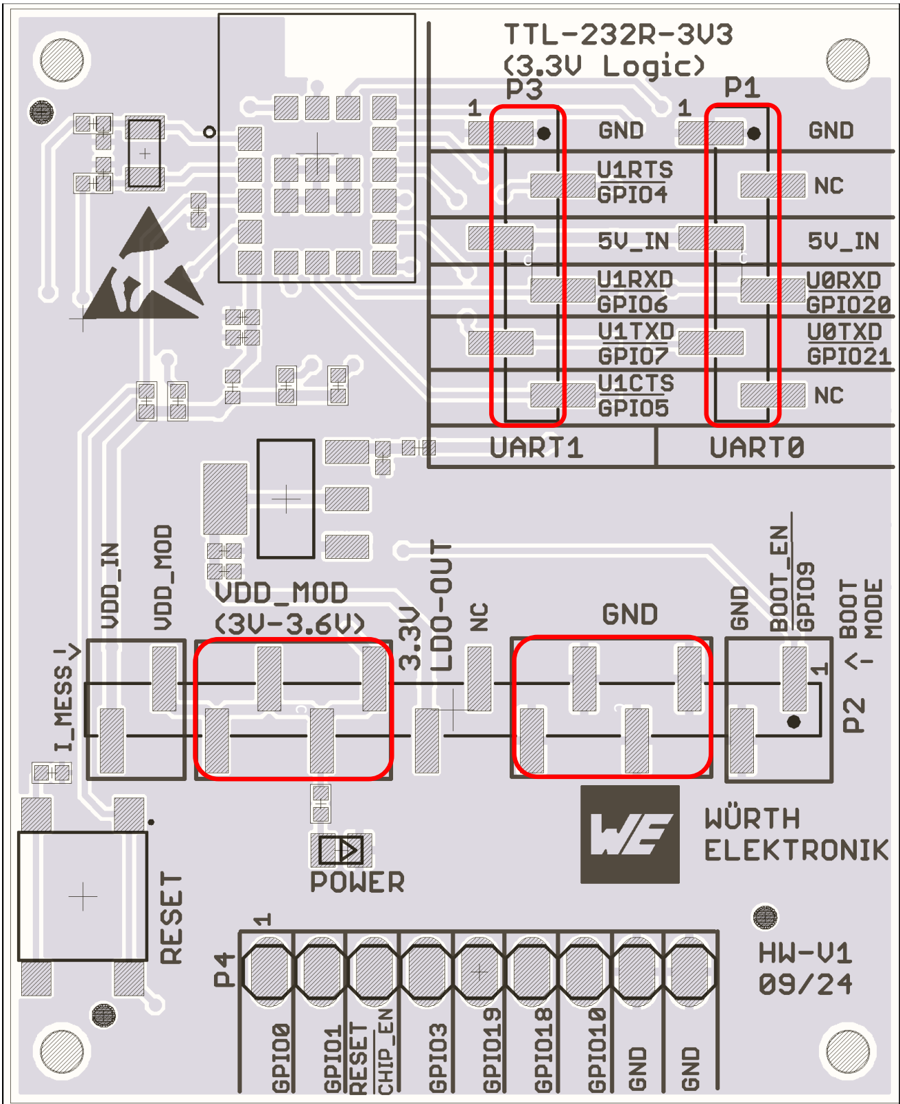
Figure 5: Connectors and ports
