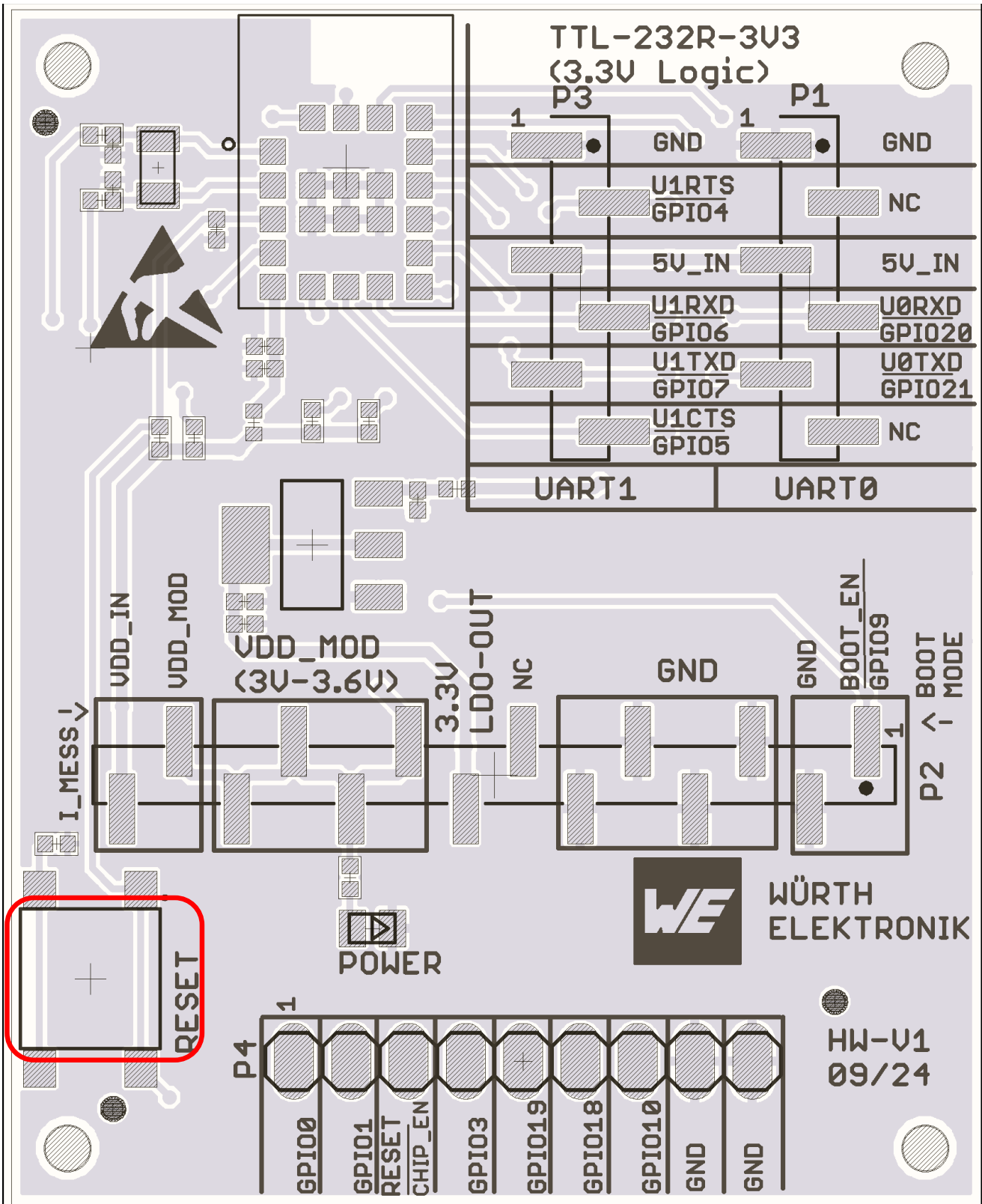
Figure 7: Buttons
