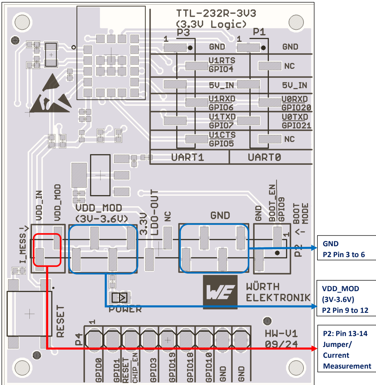
Figure 9: Setup of power supply through dedicated pins
