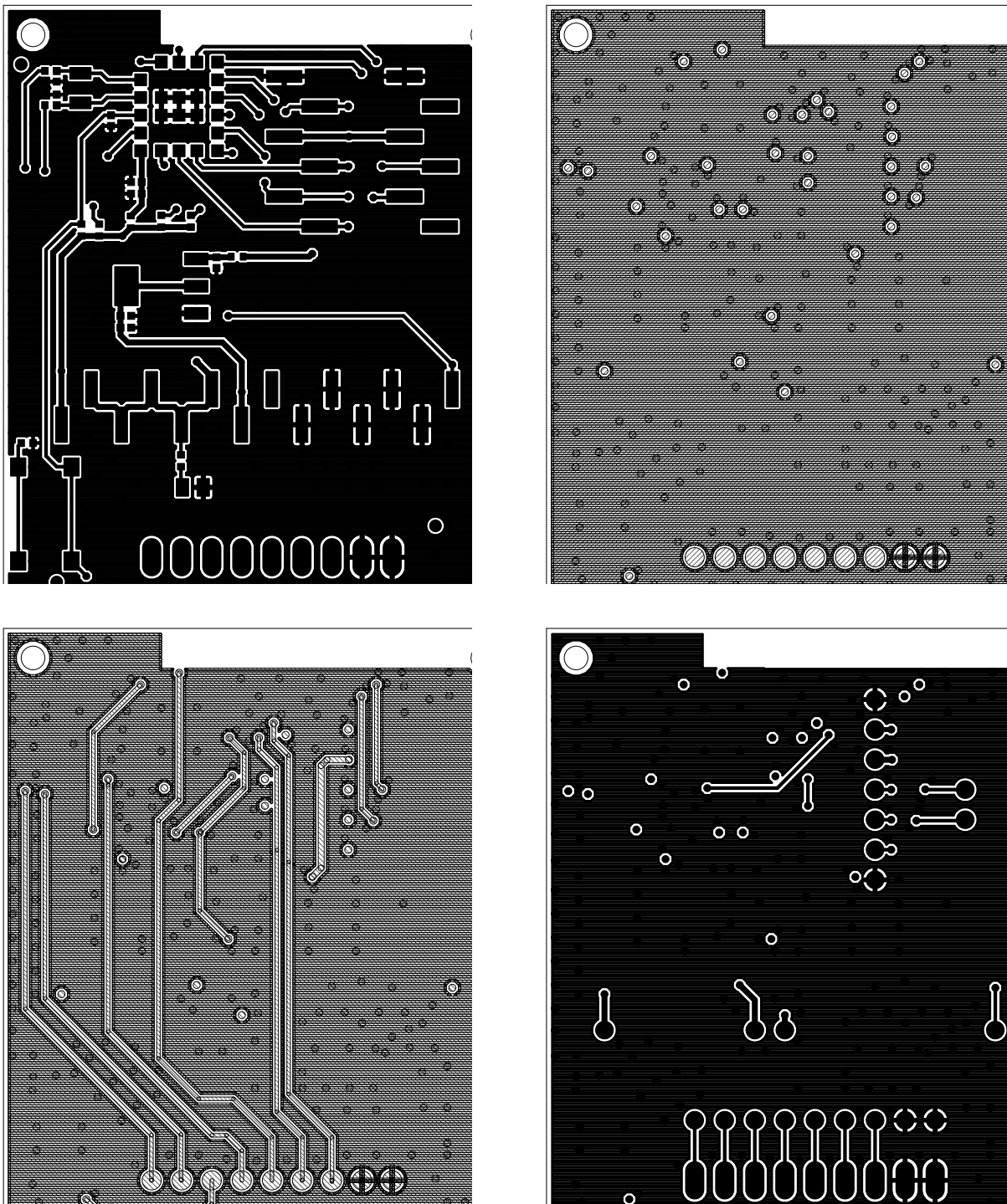
Figure 12: Top, bottom & internal layers
