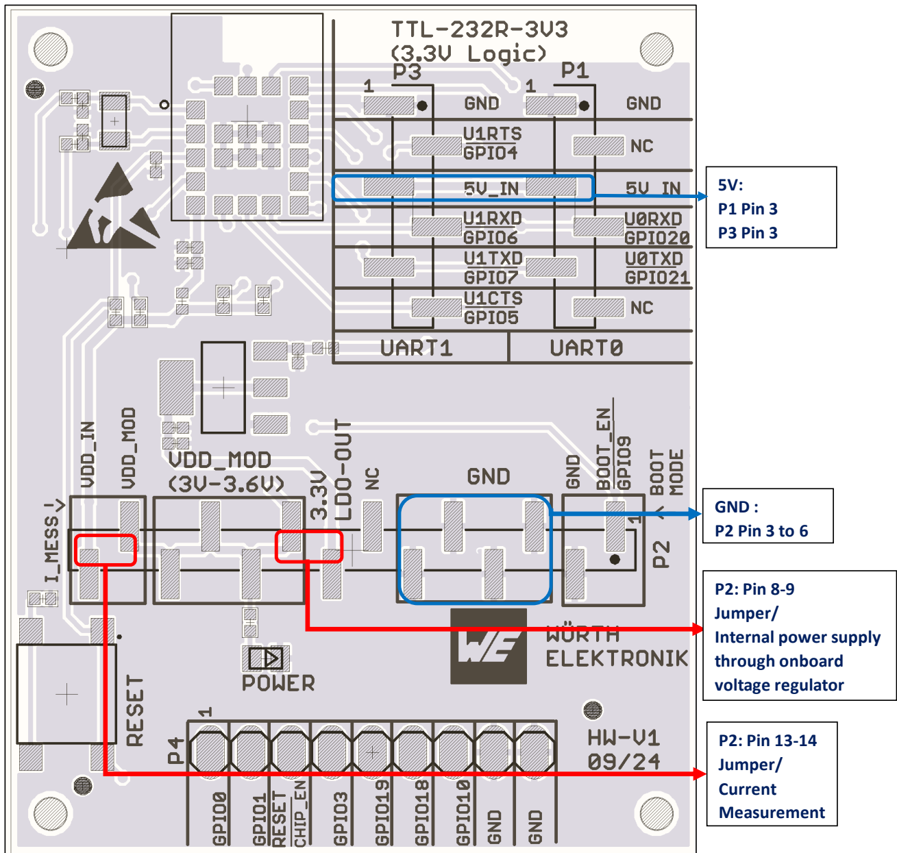
Figure 8: Setup of power supply through TTL-232R-3V3 cable
