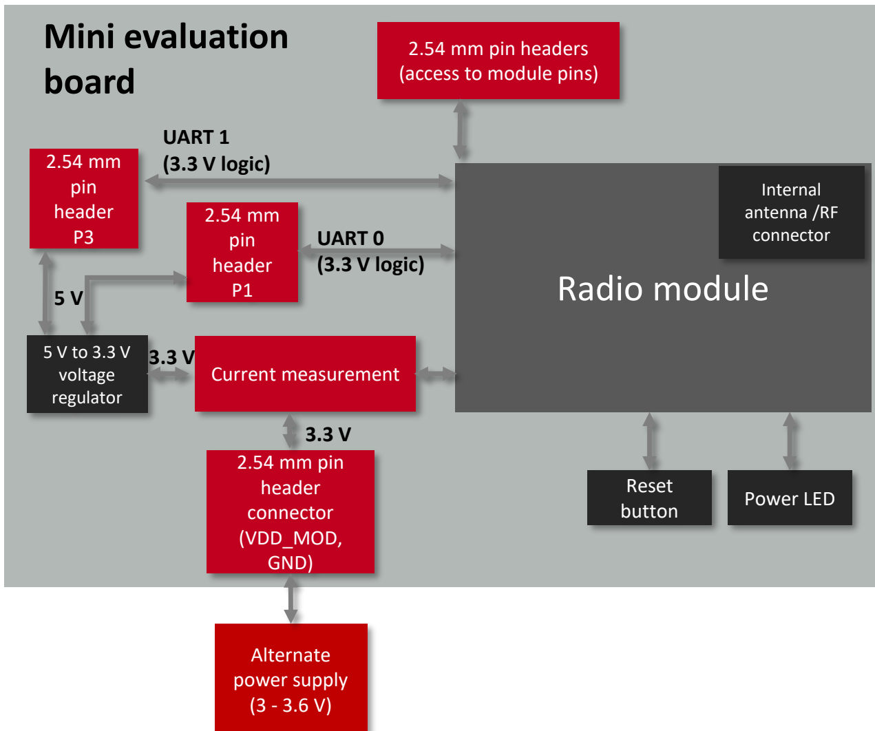
Figure 3: Block diagram of Stephano-I/Orthosie-I with internal antenna or RF connector
