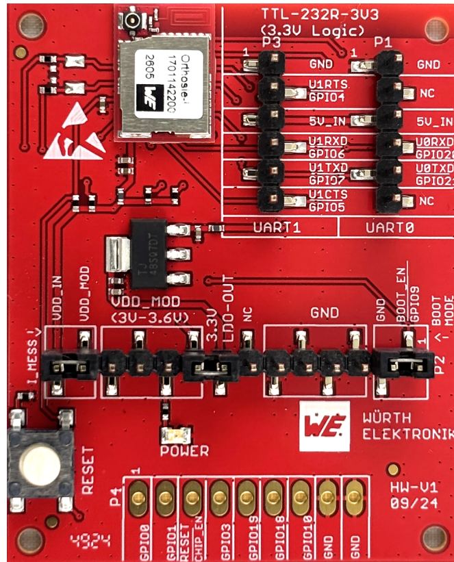
Figure 2: Orthosie-I with RF connector mini-EV-Board
