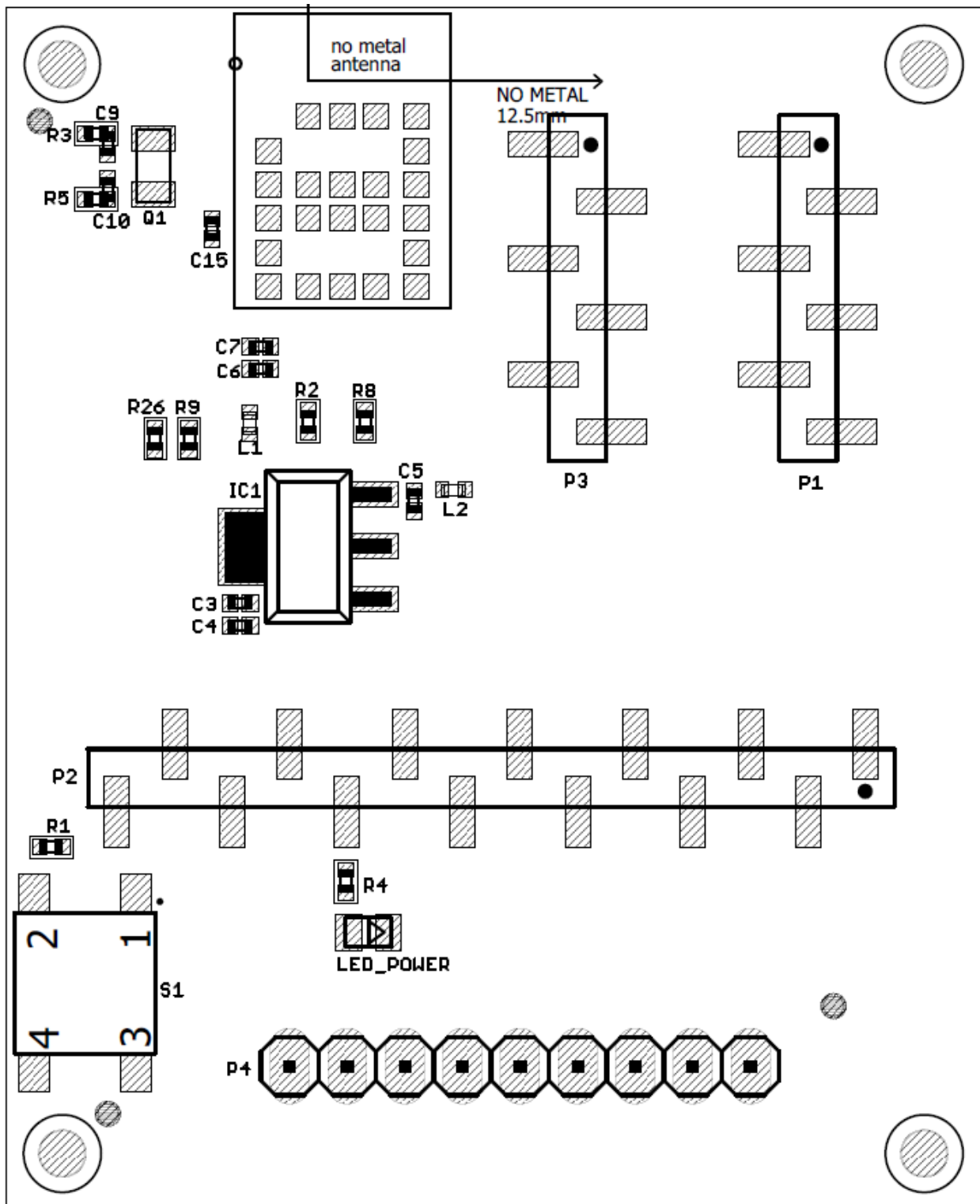
Figure 11: Assembly diagram
